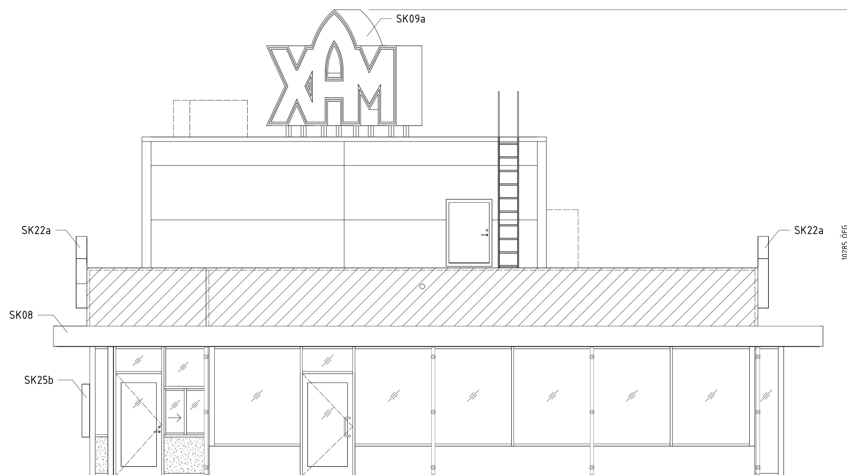
FASAD MOT DELIVERY / UTESERVERING
