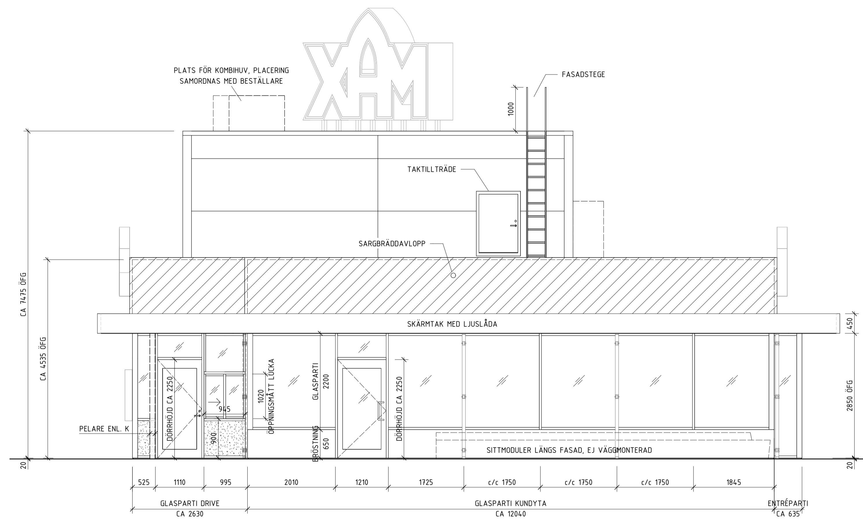
FASAD MOT DELIVERY / UTESERVERING
